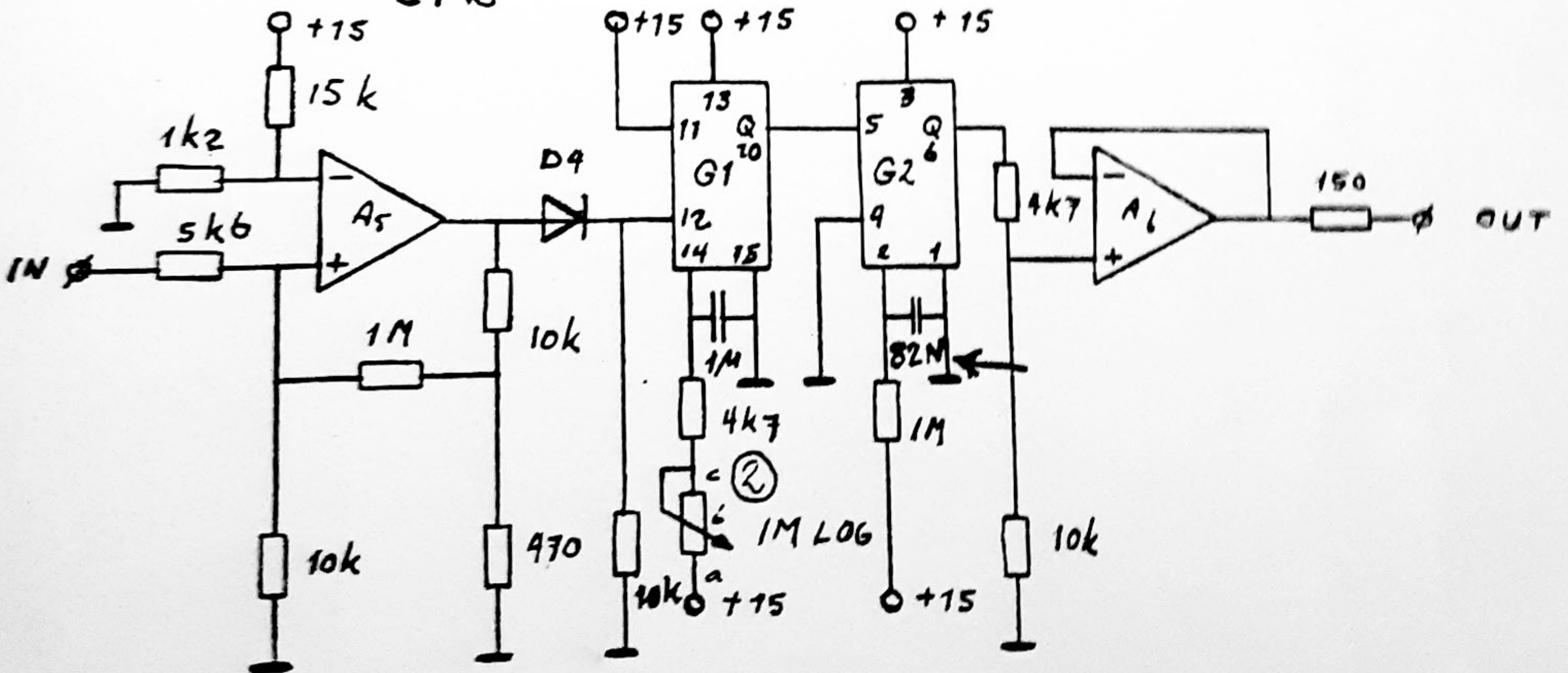
TRIGGER DELAY
