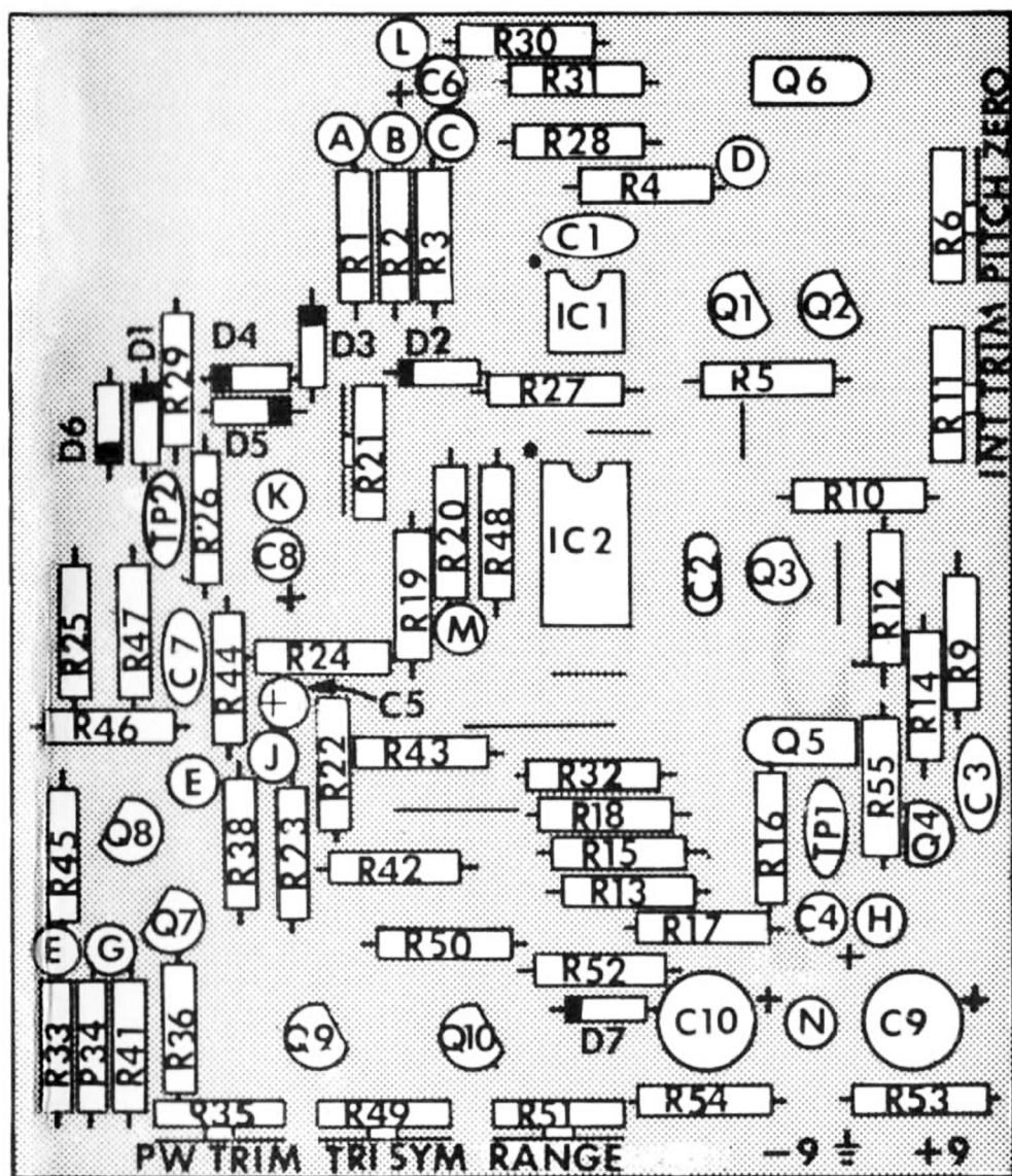
Figure 1 - Circuit board parts placement
