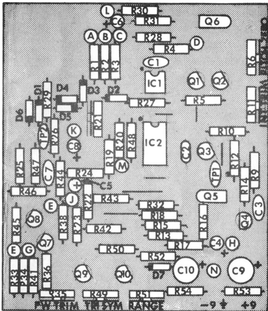
Figure 1 - Circuit board parts placement
