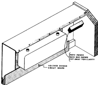
Figure 5 - Mounting the Reverb Spring
