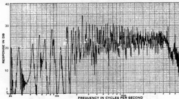
Figure 10 - Reverb Frequency Response
